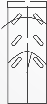
Air turn rail made of 0.6 gauge gal.iron A - 114 B - 57 C - 114 D - 83
