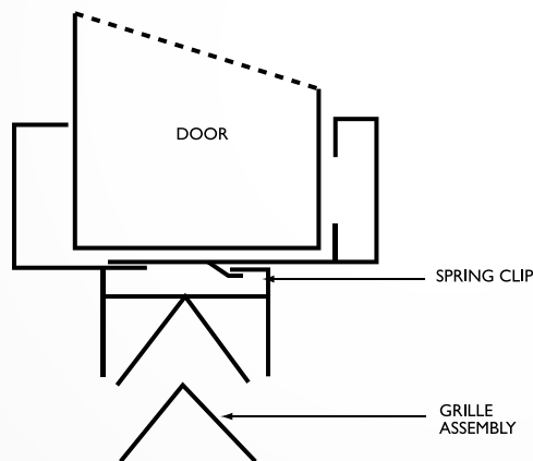
DOOR GRILLE WITH SPRING CLIP (SC) fig. 12
